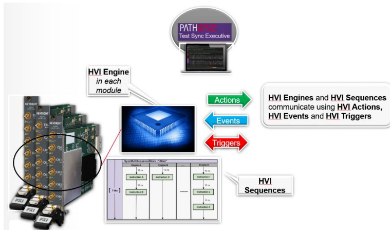
Figure 1. Hard Virtual Instrument (HVI) Elements and Operation Source: Keysight.com
